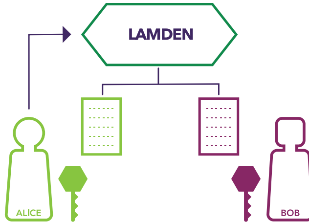
Figure 1: Alice initiates a swap by sending a message to the Ledger. The Ledger then takes the swap requirements and compiles them into Solidity bytecode to be deployed on each chain.
