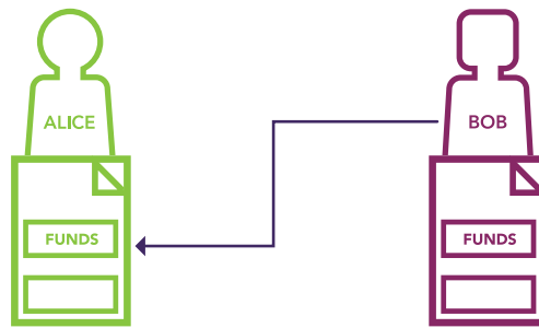
Figure 4: Assuming that this is an agreeable swap, both chains deploy the contract, and check to see if the other party has done the same by searching for the bytecode on the latest block. If this has not occurred, the chain does not have to follow through with any obligations, and the transaction reverts without loss of funds.
