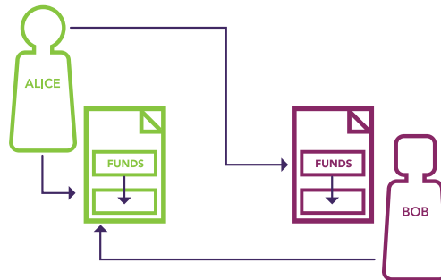
Figure 6: The best case scenario for both parties, therefore, is to resolve the payment channel on the opposing chain, and resolve the contract on their own chain as soon as possible. By adding economic incentive to do this, the network benefits from quick chain-to-chain transfers.
