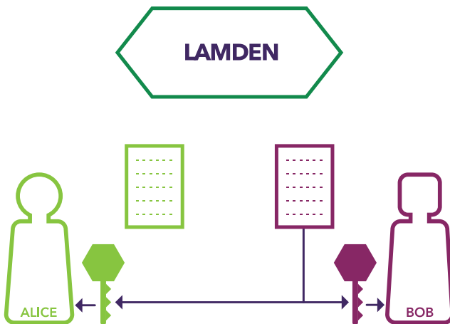
Figure 2: The bytecode is signed with each chain's public key and sent to both parties. Alice deploys their contract. Bob keeps a copy to verify later.
